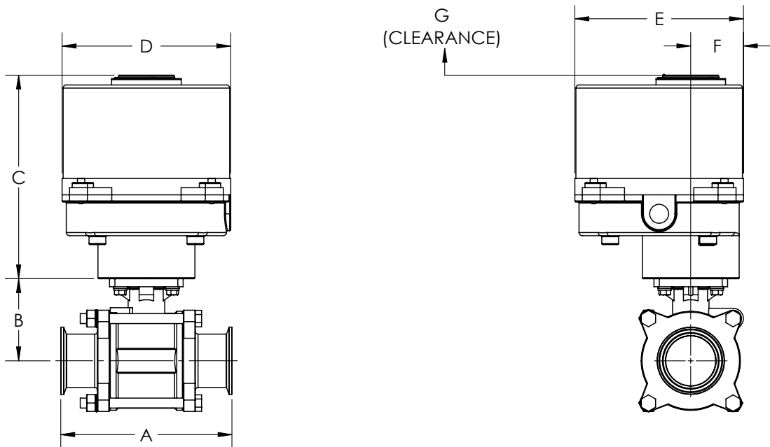
Electric Actuator - BM-2
