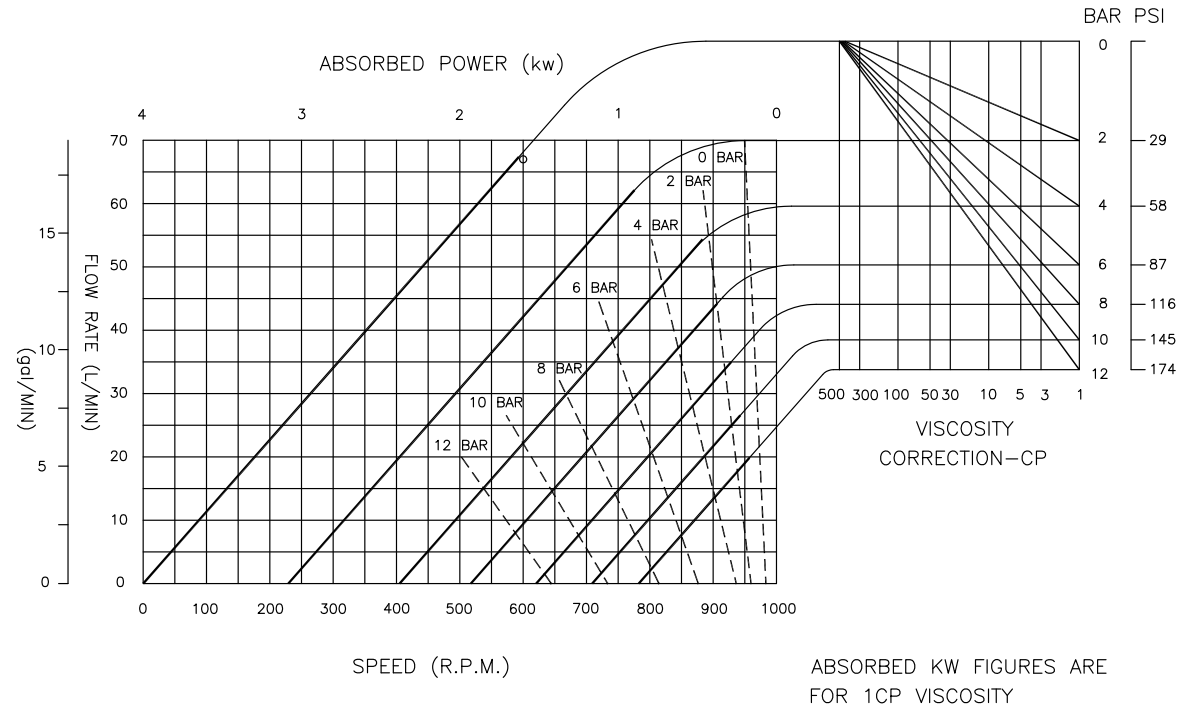
RZL 115 Heli-Lobe Capacity
