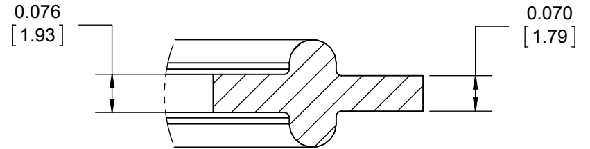
DETAIL B SCALE 4 : 1
