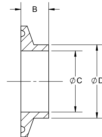
SECTION X-X
